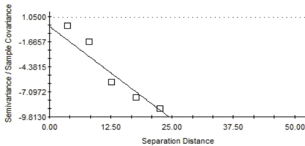
Linear model ( C_0 = -0.01 ; C_0 + C = -9.03 ; A_0 = 22.40 ; r^2 = 0.946 ; RSS = 6.13 )
